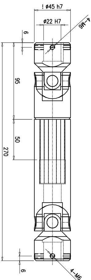
GN 808.2-45-K22-270-50 (Add tap) QTY : 1 SET
