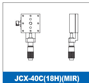
JCX-40C(18H)
