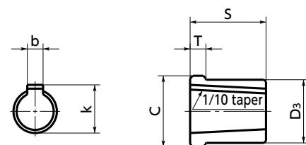
Adapter Details
